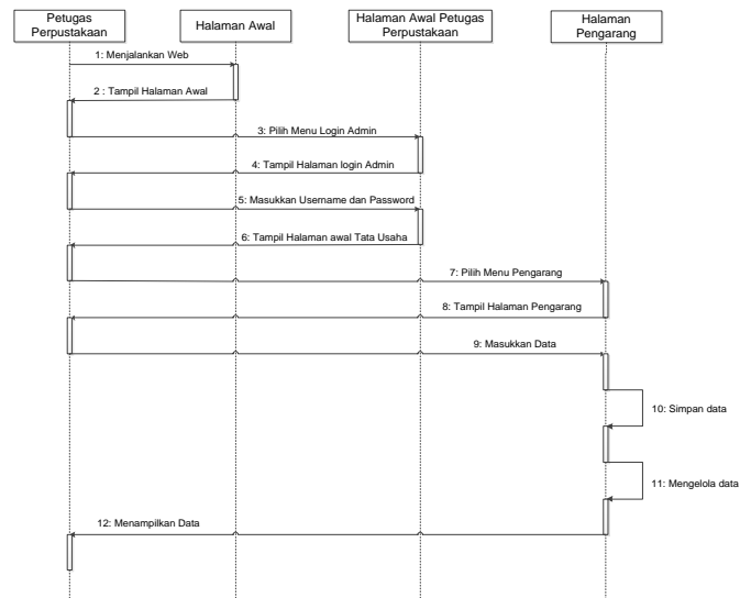
Gambar 3. Sequence Diagram Pengarang
