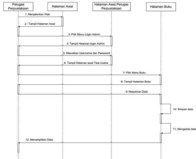
Gambar 5. Sequence Diagram Buku
